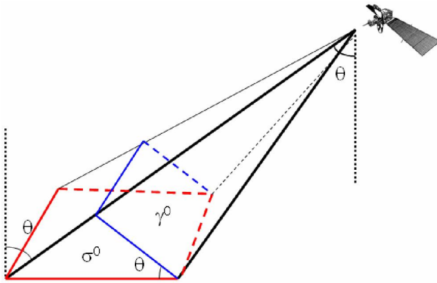
Figure 2. The relationship between the look angle ( \theta ) and the projections of backscattering coefficient on the ground range (sigma \sigma^0 ) and on the vertical plane to the slant range (gamma \gamma^0 ).
