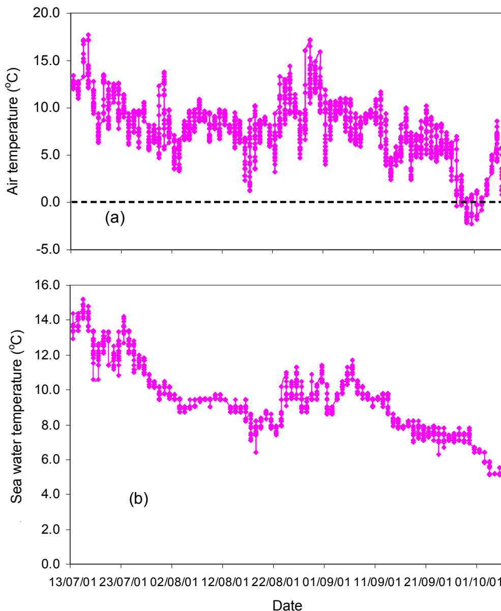
Figure 7. (a) The hourly air temperature, and (b) the hourly sea water temperature measured at the NOAA's buoy station 48011 (67°34'54"N, 164°11'06"W) from July 13, 2001 to October 6, 2001 (the daily variation of the temperature is represented by the vertical length of the line corresponding to the day).
