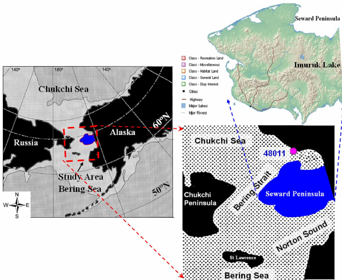
Figure 1. Study areas including Seward Peninsula and its coastal areas, which contain the Bering Strait and Norton Sound (The buoy Station 48011 of National Data Buoy Center (NDBC) of NOAA is also shown, http://www.nodc.noaa.gov/BUOY/bakw.html ).
