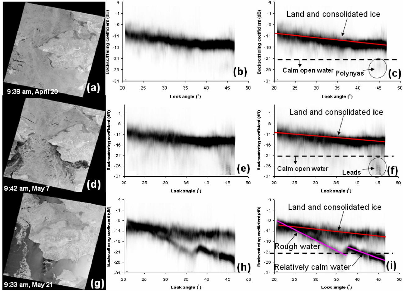
Figure 3. RADARSAT-1 ScanSAR images in descending mode (left column from top to bottom) and the feature space images (middle and right columns from top to bottom) corresponding to April 20, May 7, and May 21, 2001.
