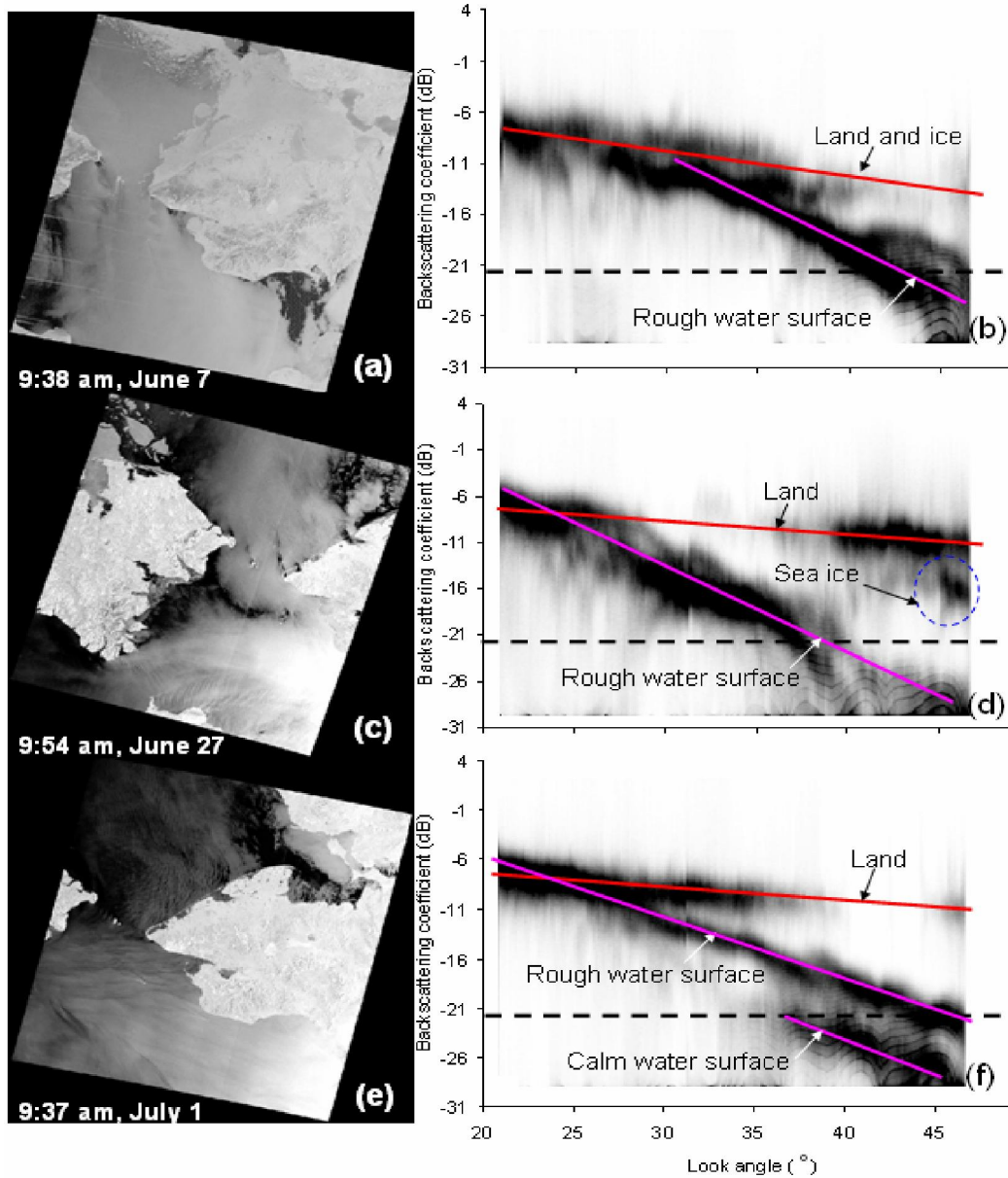
Figure 4. RADARSAT-1 ScanSAR images in descending mode (left panel from top to bottom) and the feature space images (right panels from top to bottom) corresponding to June 7, June 27, and July 1, 2001.
