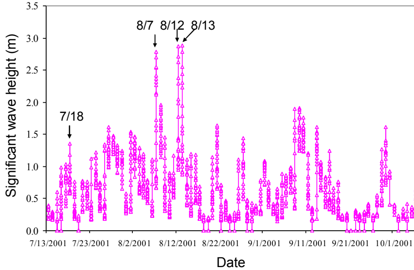
Figure 6. The hourly significant wave height measured at the NOAA’s buoy Station 48011 from July 13, 2001 to October 6, 2001 (the daily variation is represented by the vertical length of the line corresponding to the day).
