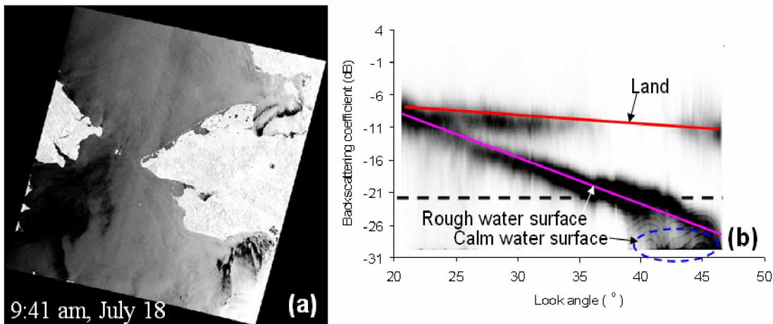
Figure 5. (a) RADARSAT-1 ScanSAR backscattering coefficient image in descending mode, and (b) the corresponding feature space image of July 18, 2001.
