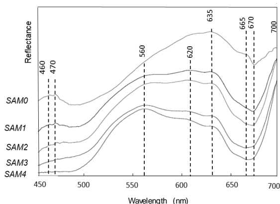
Figure 2. Reflectance spectra for the reference (uninoculated) granite block (SAM0), and blocks inoculated with dry weight biomass concentrations of 0.05 (SAM1), 0.10 (SAM2), 0.15 (SAM3), and 0.20 mg·cm -2 (SAM4).
